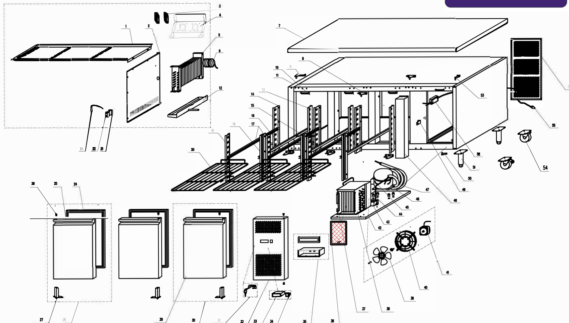
explode of RGN3100TN
